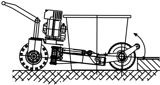
HYDRAULICALLY CLAMPS AND LIFT CONTAINERS
