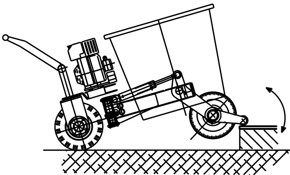
THE MACHINE IS ABLE TO MOUNT STEPS OF MORE THAN 8" HEIGHT
